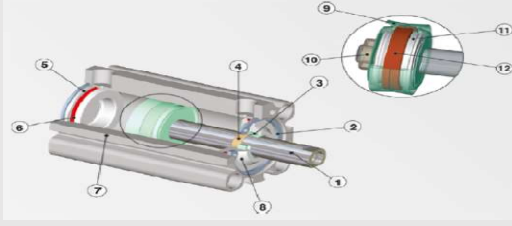
BB/BF 12 - 25
