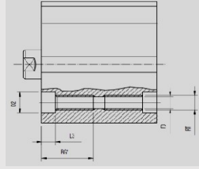
BB/BF 12 - 25
